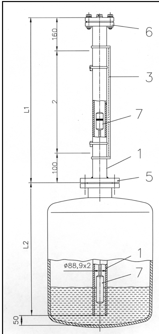
Parts drawing ITA-4.1
